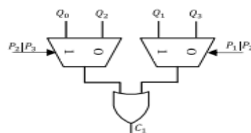
Fig.8 C1 generating circuit.
