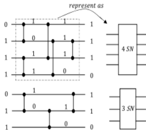
Fig.4 Three- and four-way sorting networks.
