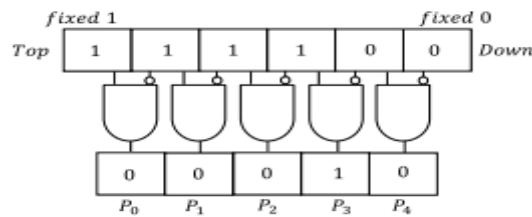
Fig. 7 One-hot code generation circuit.
