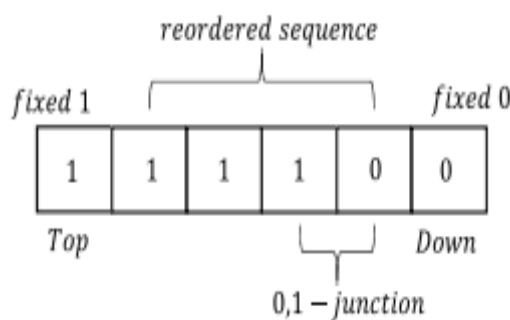
Fig.6 Definition of a sequence.
