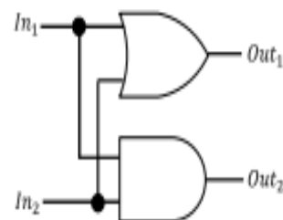
Fig.5 Two-input binary sorter
